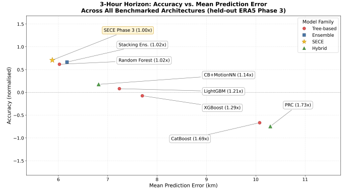
Fig. 1. Held-out 3h benchmark for the eight locked systems. Each point is computed from the pooled nine-seed held-out prediction export (results/sece_era5_envi-ron_heldout/task_a_test_predictions/seed not an illustrative sketch. The horizontal axis is mean great-circle error (km) over all scored test origins; parenthetical labels are that system’s mean divided by the SECE mean (e.g., Random Forest 6.07 km/ \approx 1.02 \times vs. SECE 5.96 km). The vertical axis is a normalised accuracy index from median error relative to the tree-based family median—Table II instead reports pooled medians with 95% bootstrap CIs (e.g., SECE 4.895 km at 3 h).
