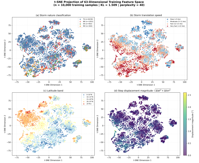
Fig. 2. t-SNE projection [30] of the 63-dimensional feature space ( n = 10,000 ), coloured by independent meteorological attributes. Coherent separation indicates the engineered features encode physically distinct regimes, which is the premise underlying the subset-expert design.
